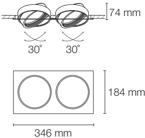
SIRIUS-R SQ DUO R111
