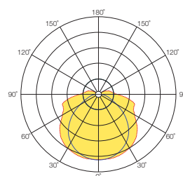
Prismatic Diffuser
